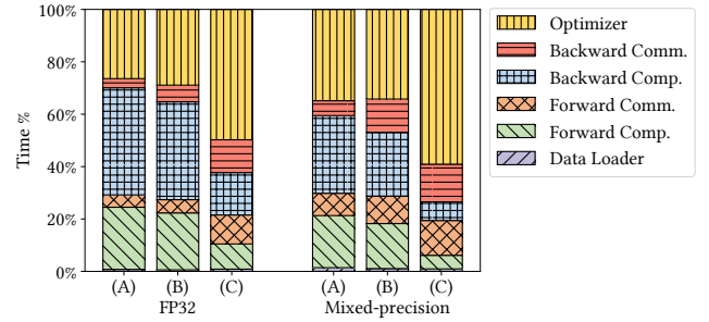
Figure 18. Performance breakdown. (A), (B), and (C) denote MoDa-1.93T , MoDa-14.5T , and MoDa-174T , respectively. FP32 and Mixed denote single- and mixed-precision training.
