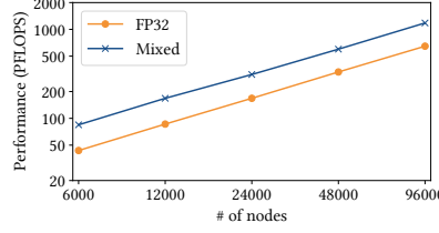
Figure 16. Weak scalability
