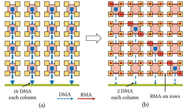
Figure 5. Memory access from CPE using DMA and RMA .
