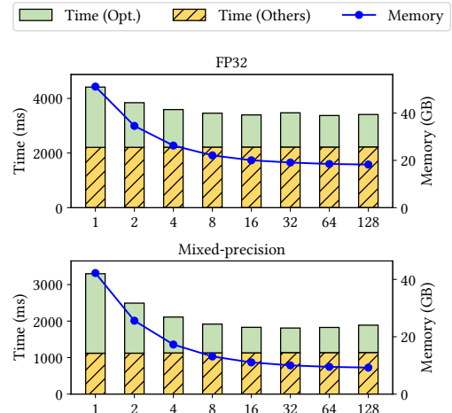
Figure 14. Time per iteration and peak memory usage at different data parallelism scales.
