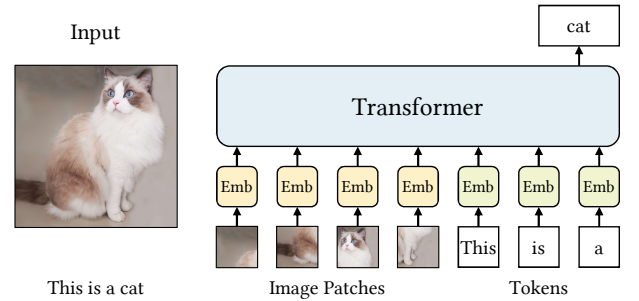
Figure 9. Demonstration of the model architecture.
