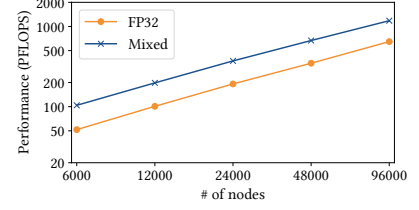
Figure 17. Strong scalability
