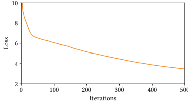
Figure 15. Loss curve
