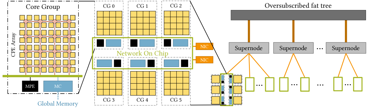
Figure 2. Architecture of the New Generation Sunway Supercomputer.
