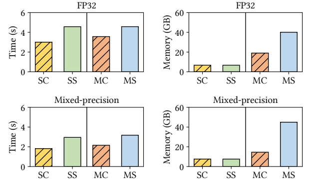
Figure 10. Time per iteration and peak memory usage in a single-node for different implementations. Note that the workload on each CG remains the same in each group of experiments.
